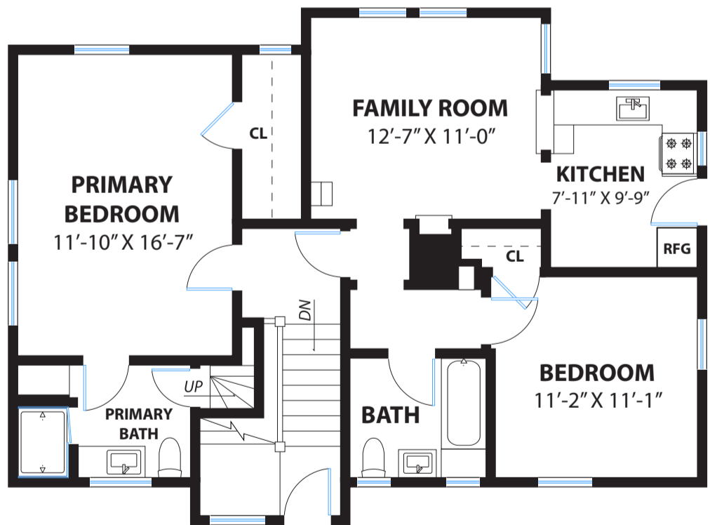
THIRD FLOOR
